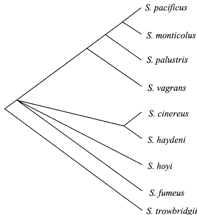
FIG. 1. Phylogeny of nine species of Sorex shrews used in this study (based on Fumagalli et al. 1999).
