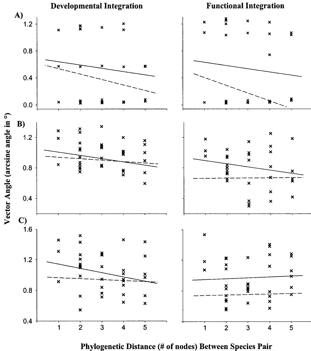
FIG. 4. The relationship between rank phylogenetic relatedness and arcsine-transformed vector angles for (A) PC1, (B) PC2, and (C) PC3 for developmental and functional integration for all species pair comparisons. Between-species vector angle reflects concordance of species pair integration pattern with larger vector angles indicating increased discordance of integration patterns. Solid lines indicate regression line for observed relationship between phylogenetic relatedness and morphological similarity. Dashed lines indicate regression line of relationship after removing the effects of phylogeny. For all graphs, observed and simulated data share the same slope indicating that more closely related species are not more similar in patterns of developmental or functional integration.
