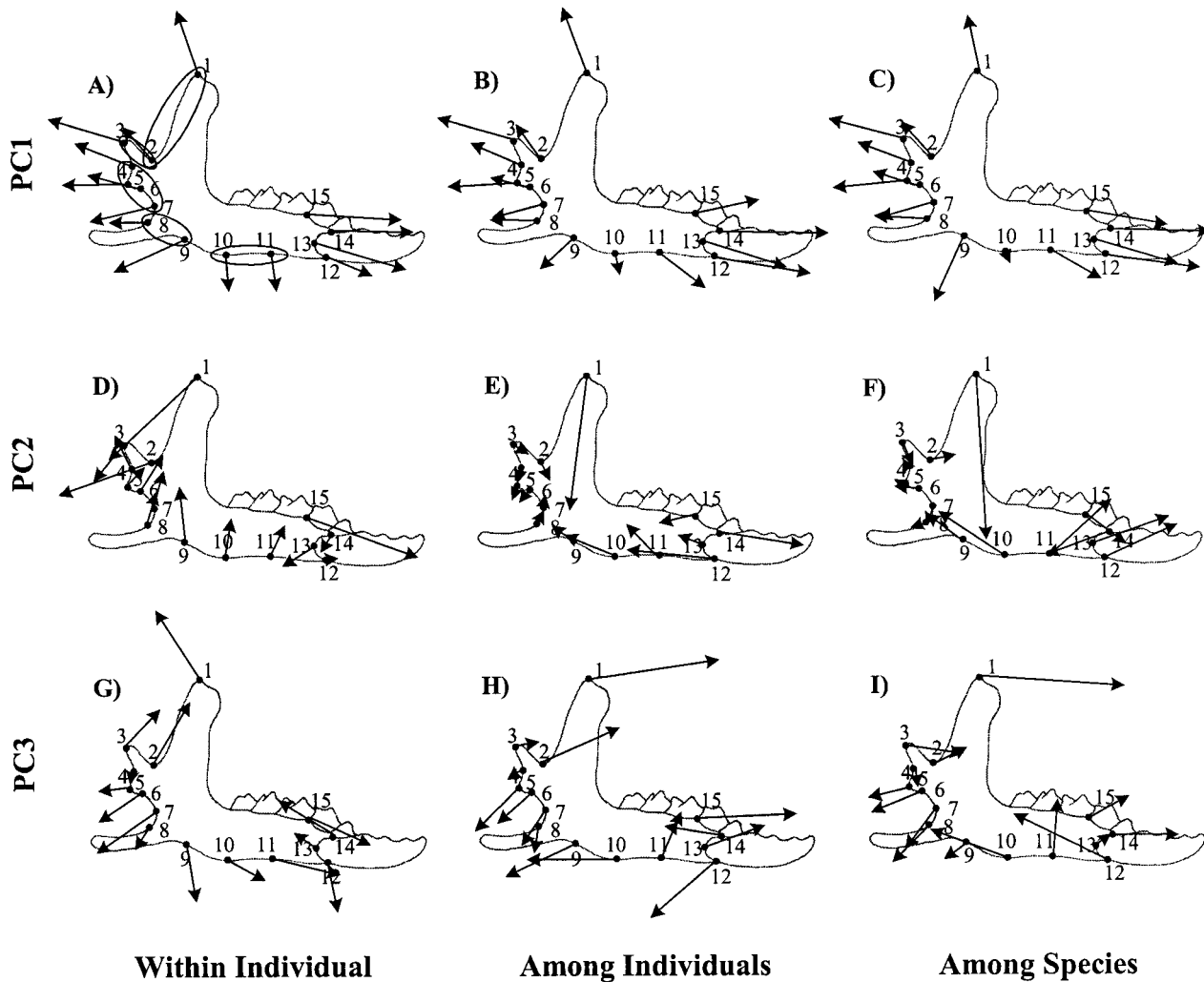
FIG. 2. Fifteen homologous landmarks describing mandible shape. (A–C) First principal components (PC1) of the covariance matrix of landmark displacement due to variation within individual (i.e., fluctuating asymmetry), among-individuals, and among-species respectively. (D–F) Second principal components (PC2) of the covariance matrix of landmark displacement due to variation within individual, among individuals, and among-species. (G–I) Third principal components (PC3) of the covariance matrix of landmark displacement due to variation within individual, among-individuals, and among species. Vector length is multiplied by 10 for better visibility. Ellipsoids indicate functionally integrated landmarks (i.e., muscle or connective tissue attachment sites).
